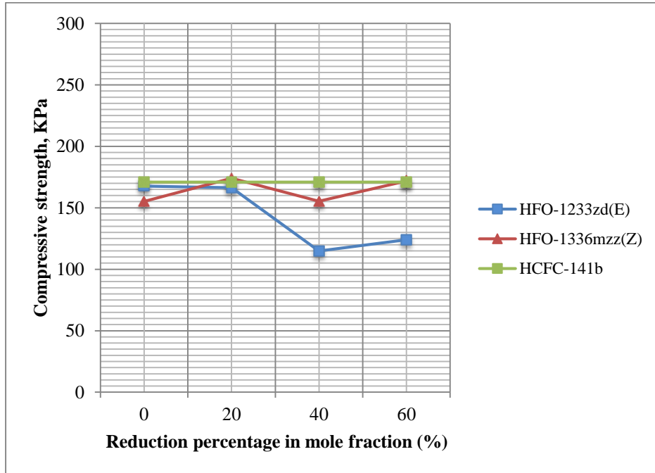
Figure 16. Compressive strength (2 months) vs. Reduction percentage in HFO mole fraction
