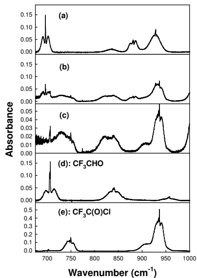
Fig. 4. Infrared spectra acquired before (a) and after (b) UV irradiation of 6.6 mTorr trans-CF 3 CH=CHF and 109 mTorr Cl 2 in 700 Torr of air diluent. Panel (c) shows the residual IR features after subtraction of trans-CF 3 CH=CHF from panel (b) . Panels (d) and (e) show reference spectra of CF 3 CHO and CF 3 C(O)Cl, respectively.
